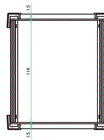
C-C (1:2.5)
